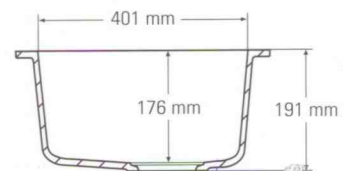
Side cross-section
