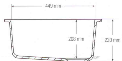
Side cross-section
