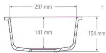
Side cross-section
