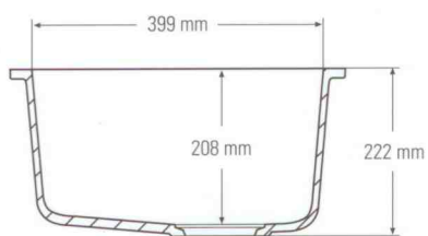
Side cross-section
