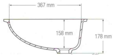
Side cross-section
