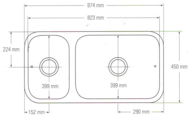
Top view * overflow
