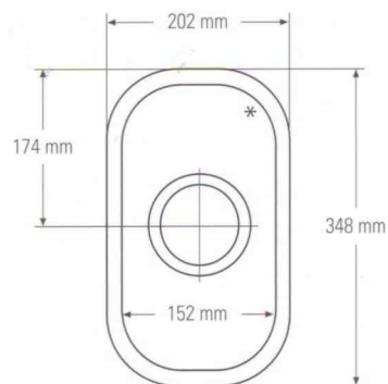
Top view * overflow
