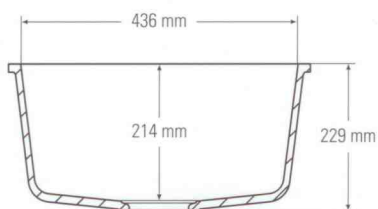
Side cross-section
