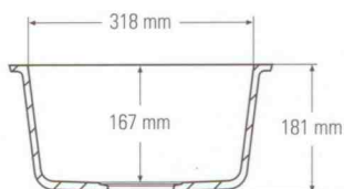
Side cross-section
